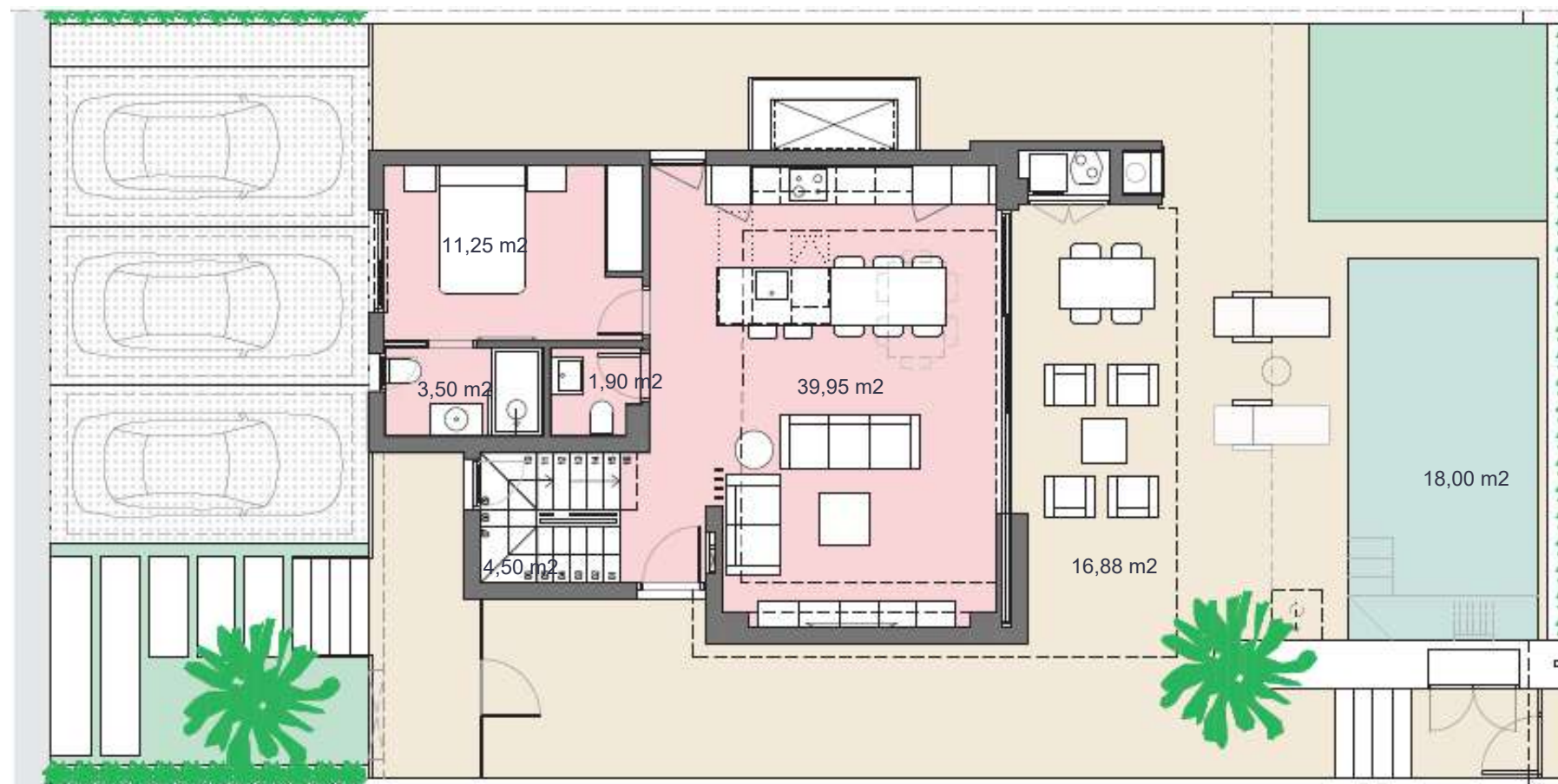
GROUND FLOOR
