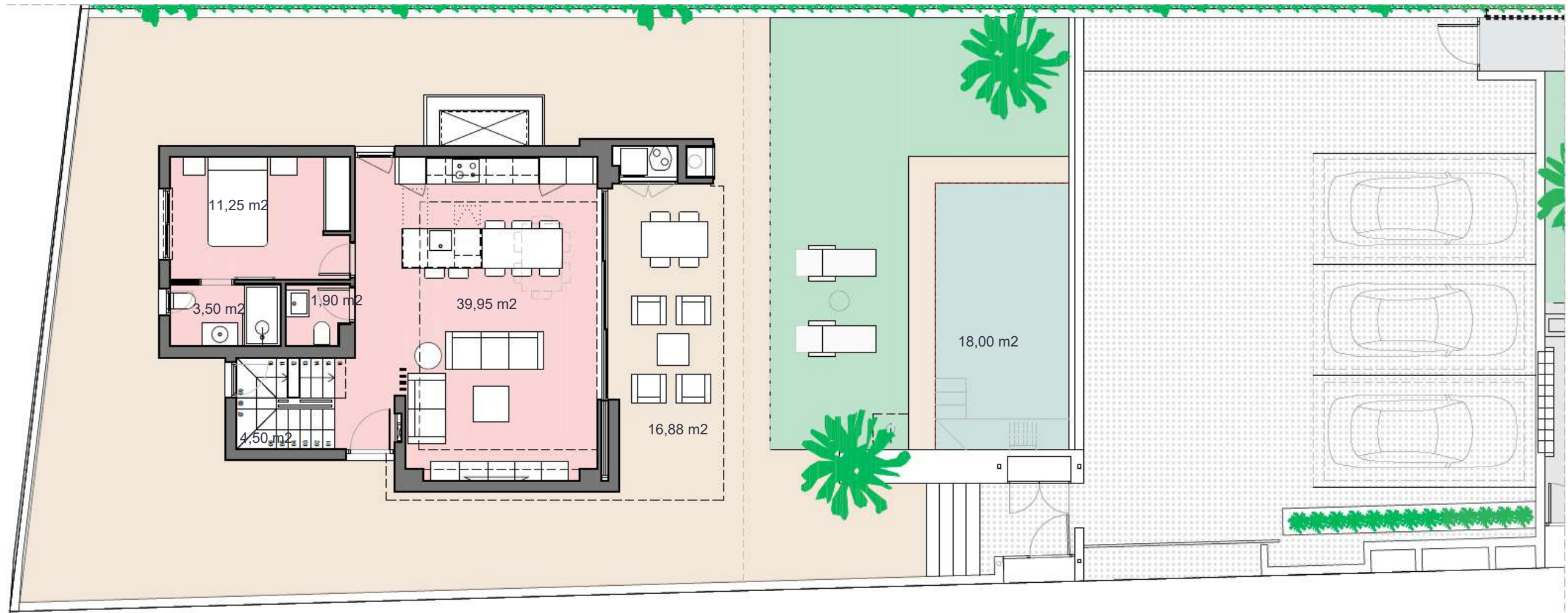
GROUND FLOOR
