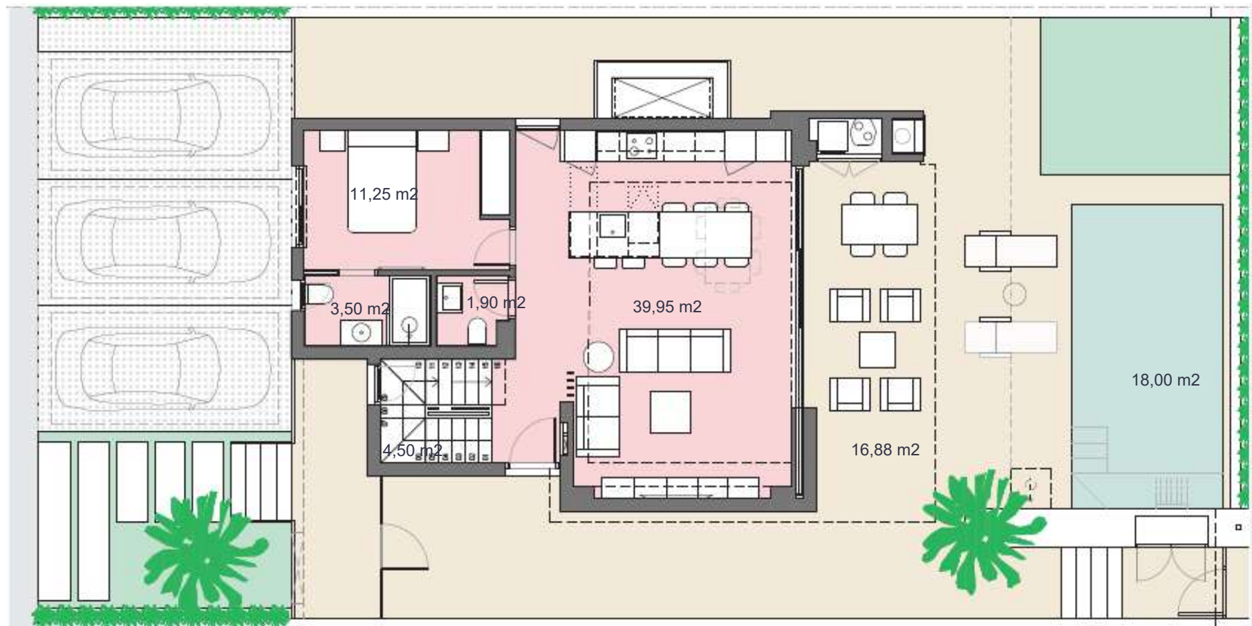
GROUND FLOOR
